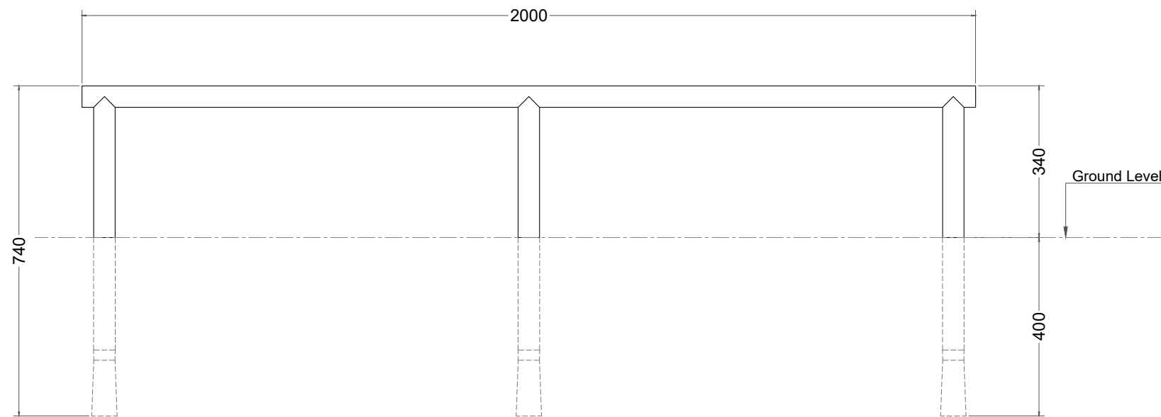
Front View
