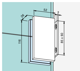
Side Connector Ref: 01.153
