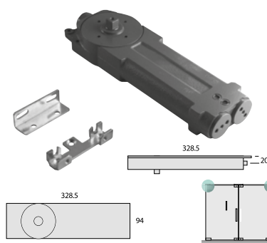
RTS 85 Transom Closer
