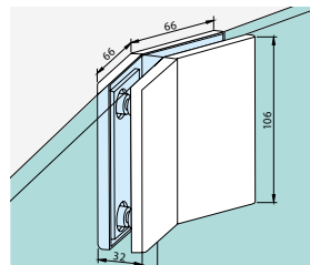
135° Connector Ref: PT80.35
