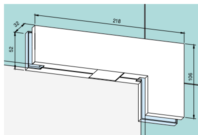
Blank Patch for Overpanel & Sidelight
