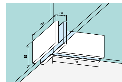
Overpanel Connector
