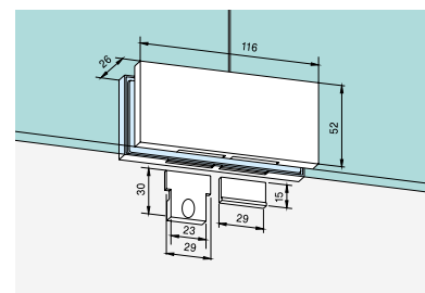
Overpanel Connector
