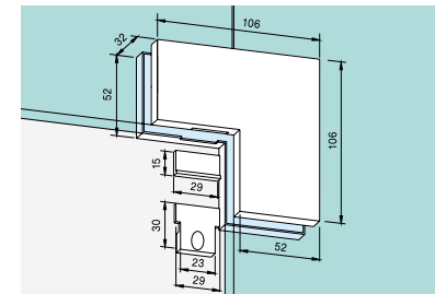
Connector
