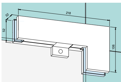
Patch for Overpanel & Sidelight
