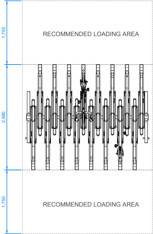
Top View Scale 1:60
