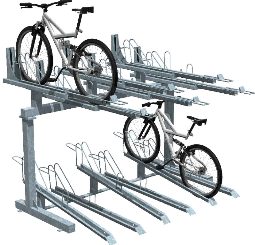
Perspective View
