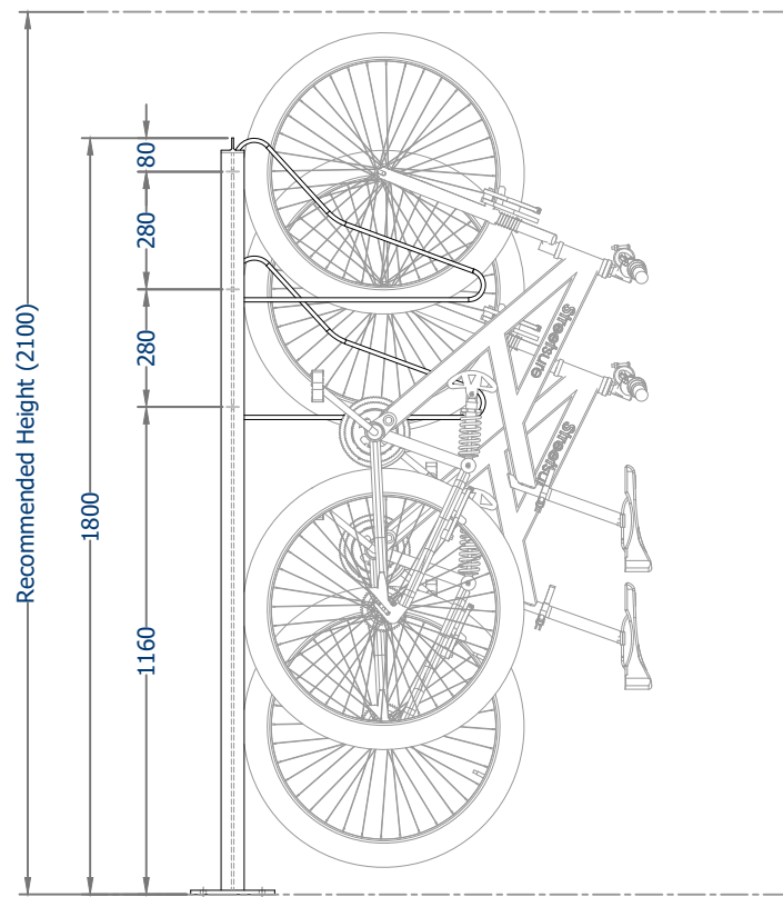
Side View
