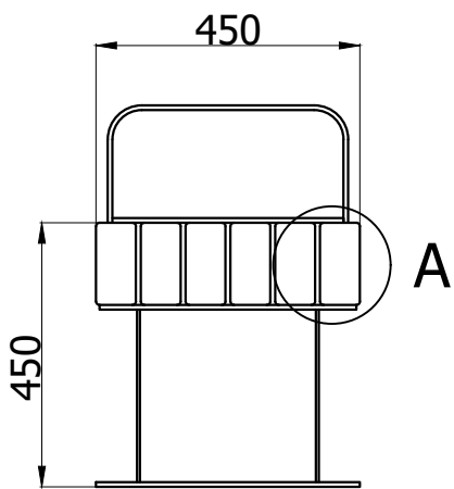
SIDE VIEW ( 1 : 14 )
