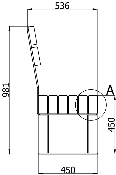
SIDE VIEW ( 1 : 14 )
