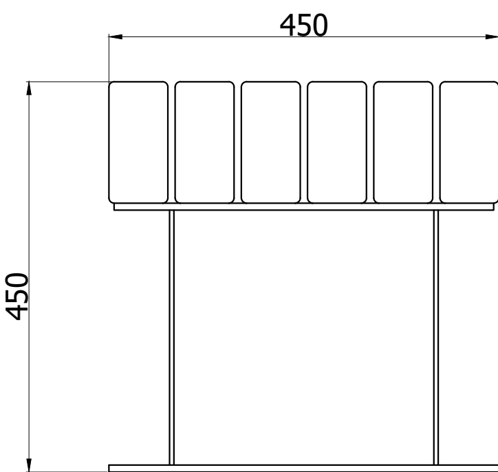
SIDE VIEW ( 1 : 6 )
