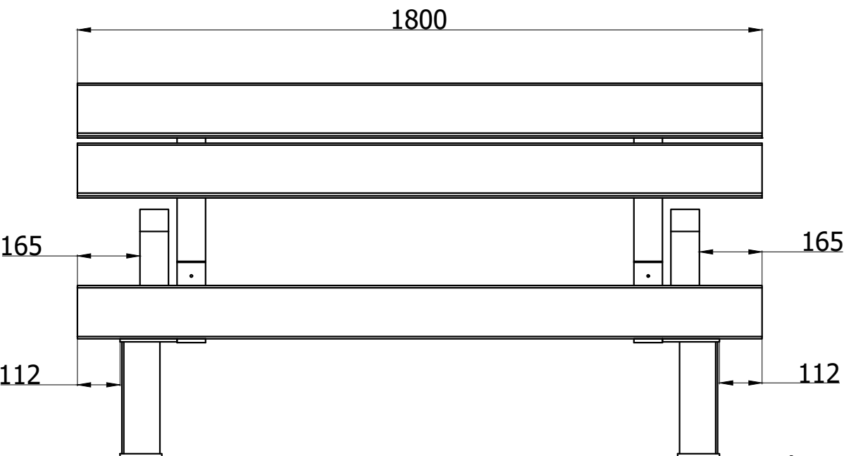
FRONT VIEW ( 1 : 14 )
