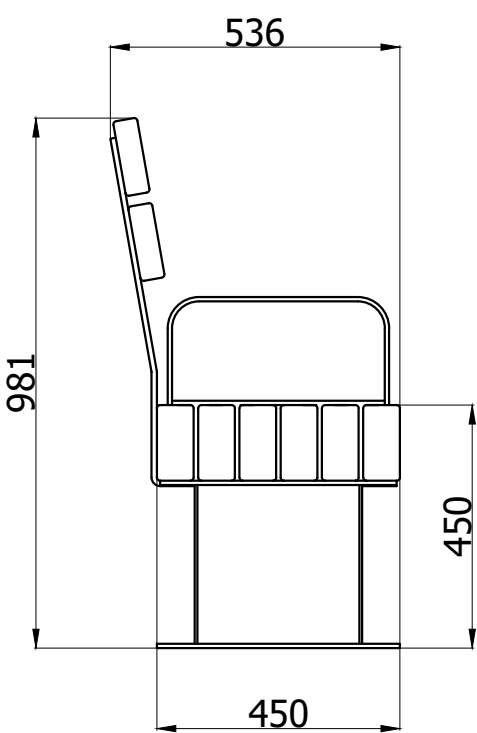
SIDE VIEW ( 1 : 14 )
