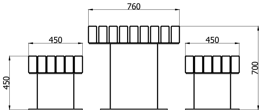
SIDE VIEW ( 1 : 18 )
