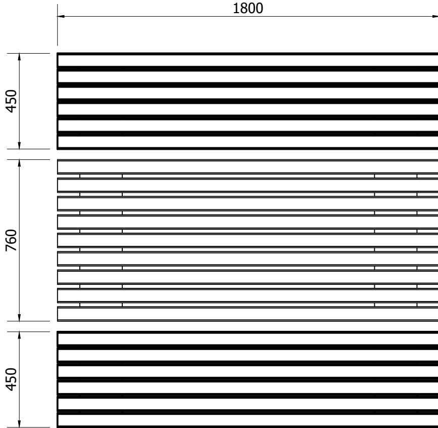
TOP VIEW ( 1 : 18 )
