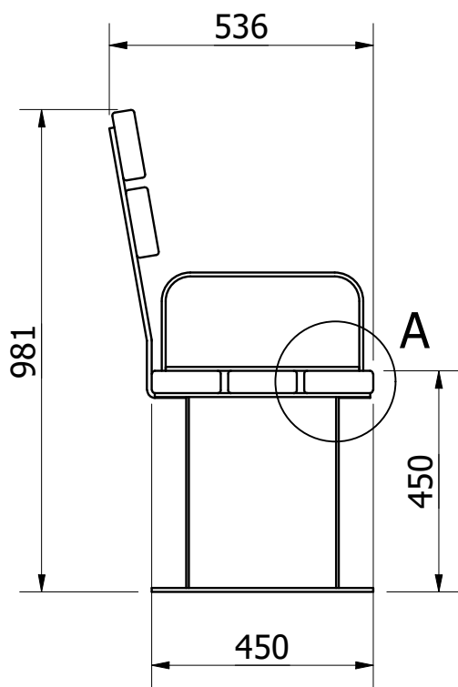
SIDE VIEW ( 1 : 14 )
