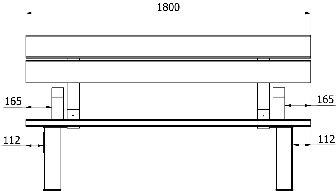
FRONT VIEW ( 1 : 14 )
