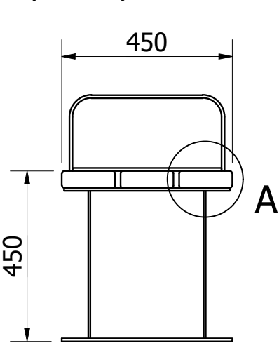
SIDE VIEW ( 1 : 14 )
