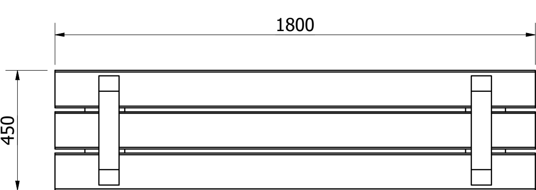
TOP VIEW ( 1 : 14 )
