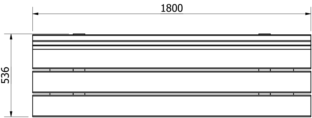
TOP VIEW ( 1 : 14 )
