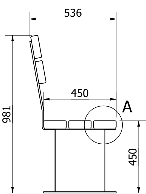
SIDE VIEW ( 1 : 14 )
