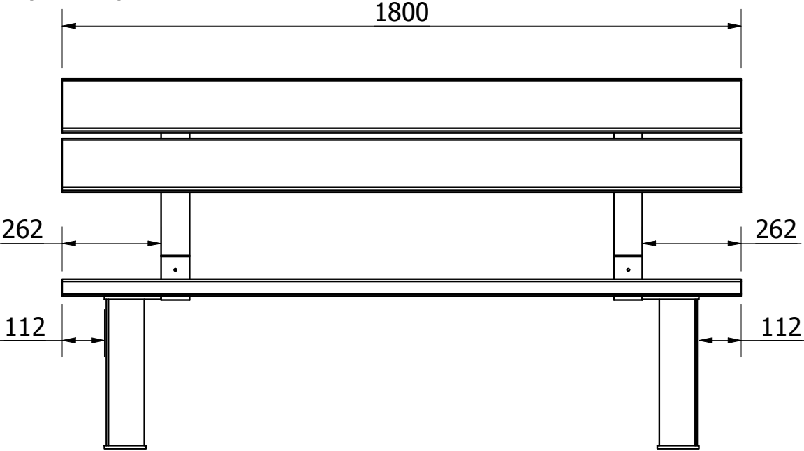
FRONT VIEW ( 1 : 14 )
