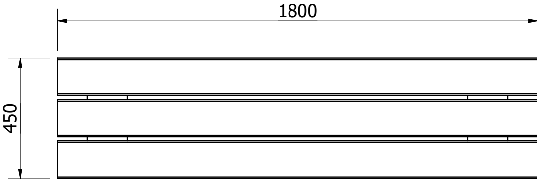
TOP VIEW ( 1 : 14 )
