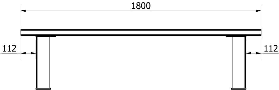
FRONT VIEW ( 1 : 14 )
