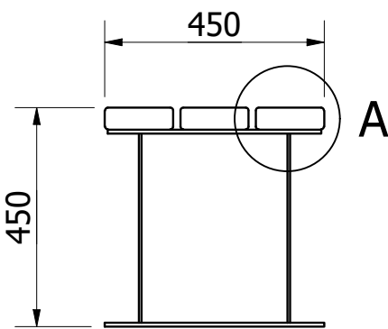
SIDE VIEW ( 1 : 14 )
