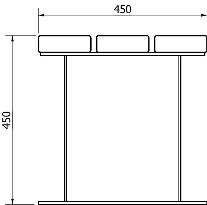
SIDE VIEW ( 1 : 6 )
