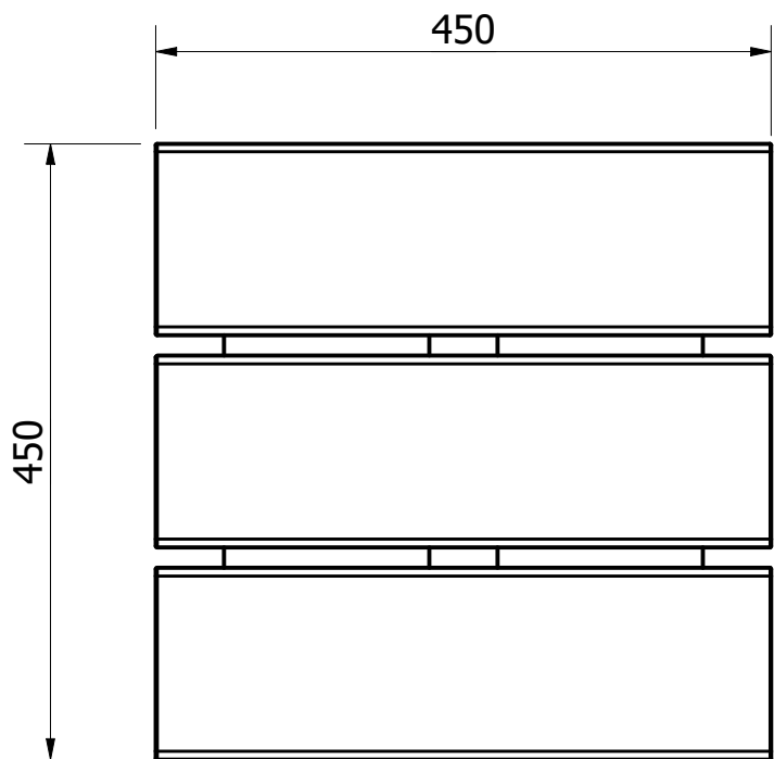
TOP VIEW ( 1 : 6 )
