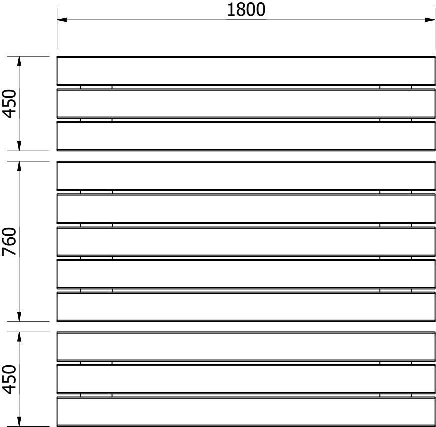
TOP VIEW ( 1 : 18 )
