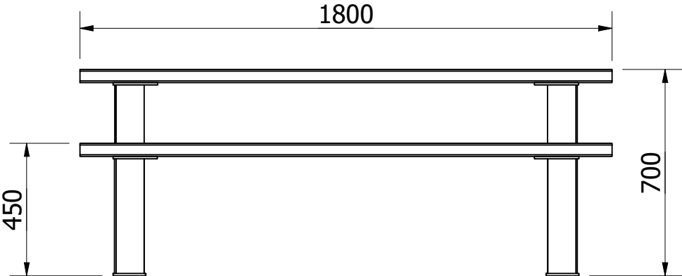
FRONT VIEW ( 1 : 18 )
