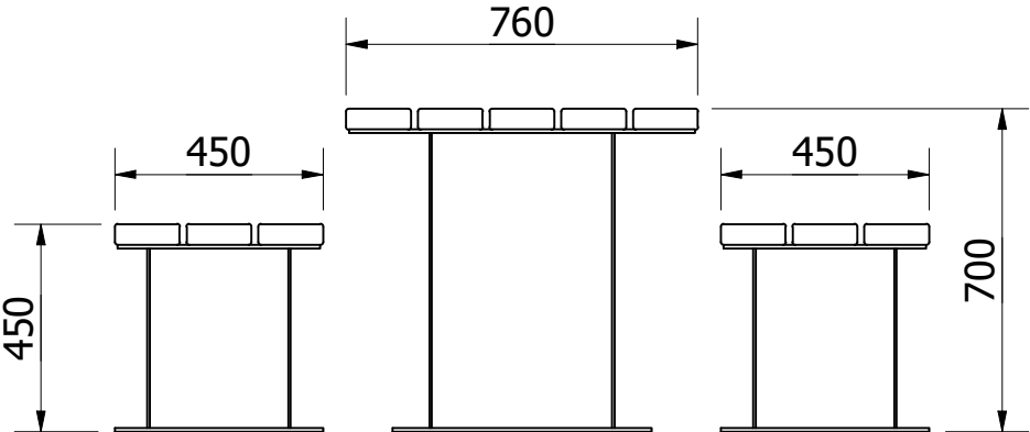
SIDE VIEW ( 1 : 18 )
