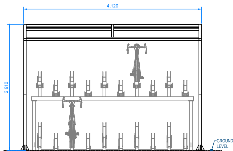
Front View Scale 1:50
