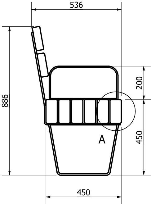
SIDE VIEW ( 1 : 14 )
