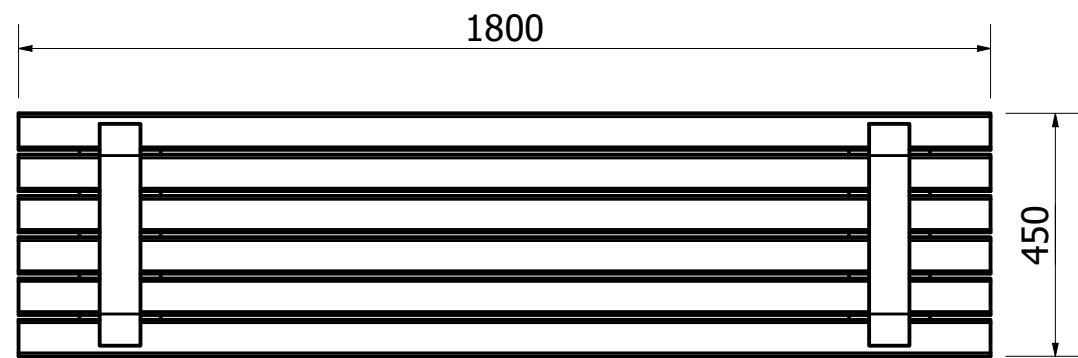
TOP VIEW ( 1 : 14 )
