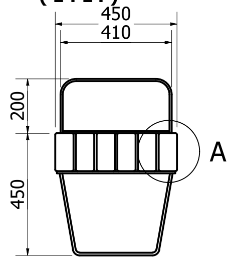
SIDE VIEW ( 1 : 14 )
