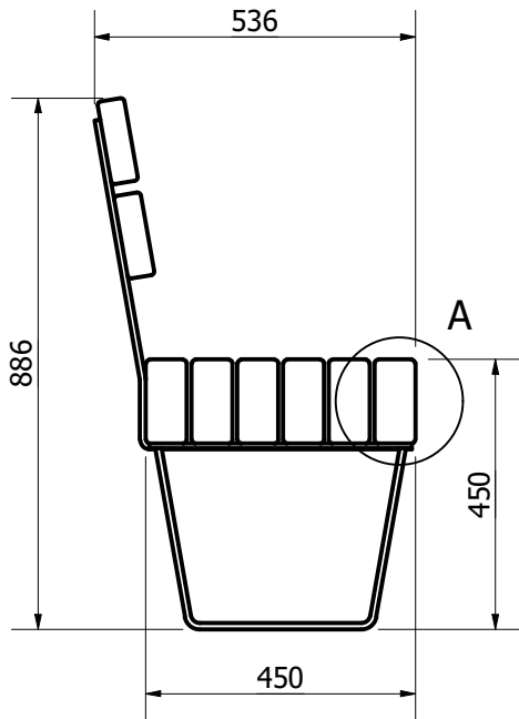
SIDE VIEW ( 1 : 14 )
