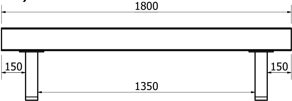
FRONT VIEW ( 1 : 14 )
