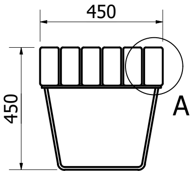
SIDE VIEW ( 1 : 14 )
