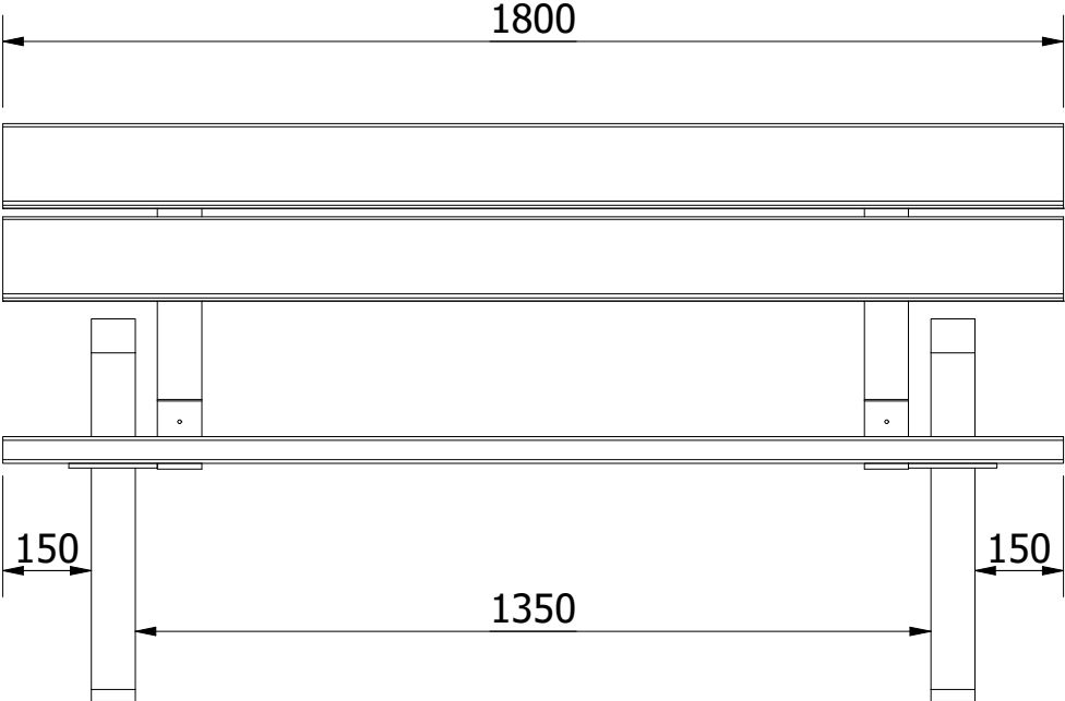
FRONT VIEW ( 1 : 14 )
