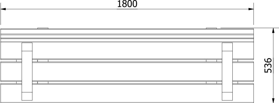
TOP VIEW ( 1 : 14 )
