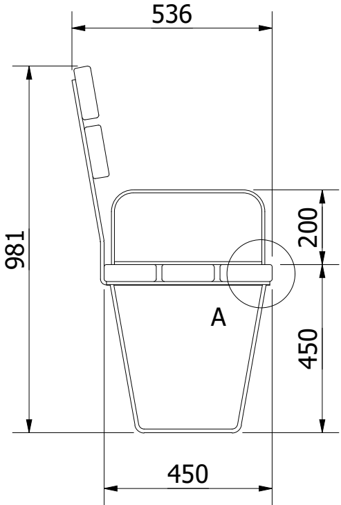
SIDE VIEW ( 1 : 14 )
