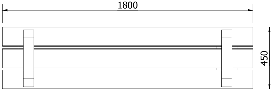
TOP VIEW ( 1 : 14 )
