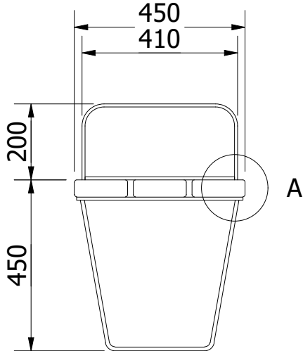
SIDE VIEW ( 1 : 14 )
