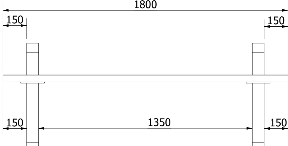
FRONT VIEW ( 1 : 14 )
