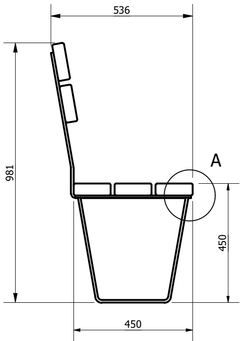
SIDE VIEW ( 1 : 14 )
