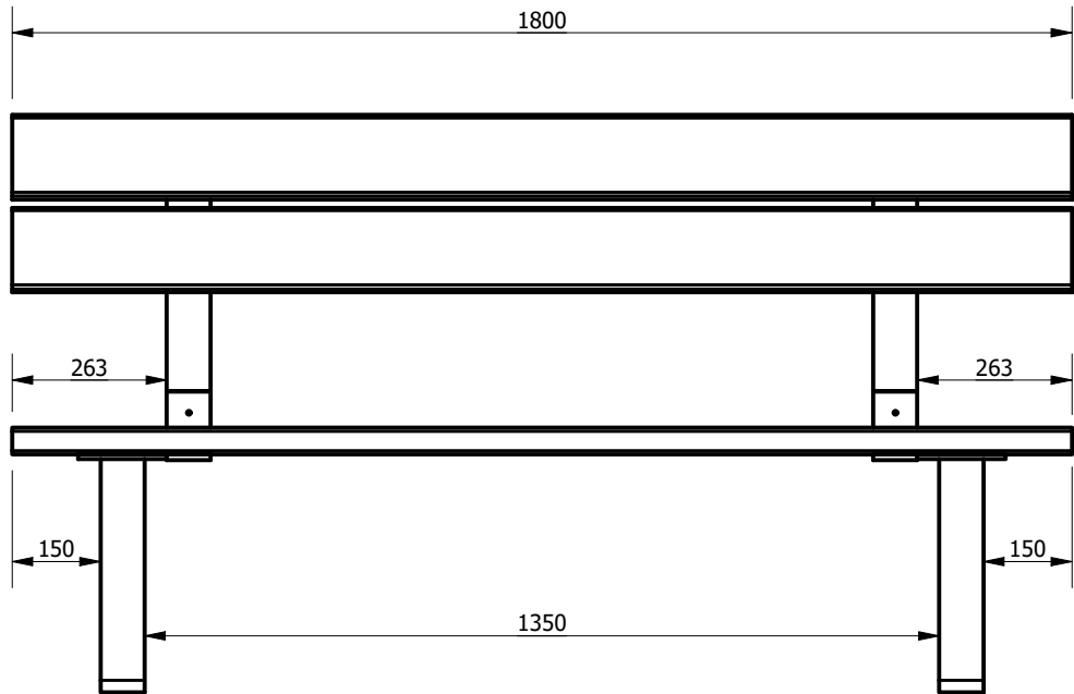
FRONT VIEW ( 1 : 14 )
