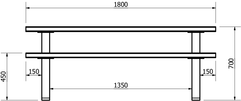
FRONT VIEW ( 1 : 18 )
