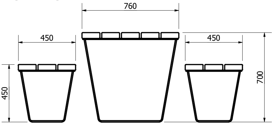
SIDE VIEW ( 1 : 18 )
