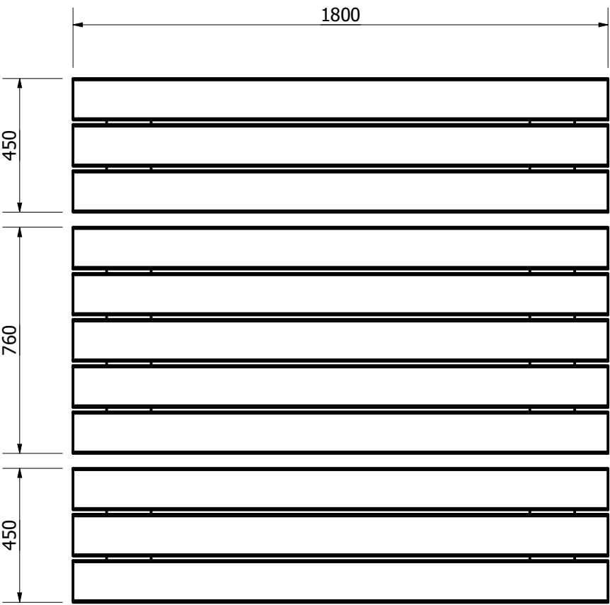
TOP VIEW ( 1 : 18 )
