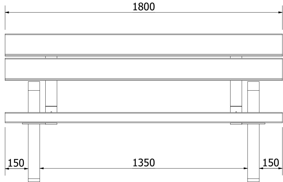
FRONT VIEW ( 1 : 14 )
