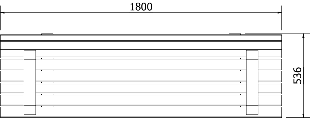
TOP VIEW ( 1 : 14 )
