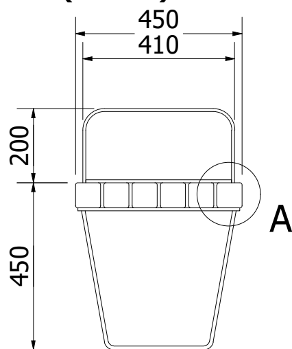
SIDE VIEW ( 1 : 14 )
