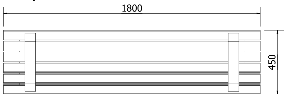
TOP VIEW ( 1 : 14 )
