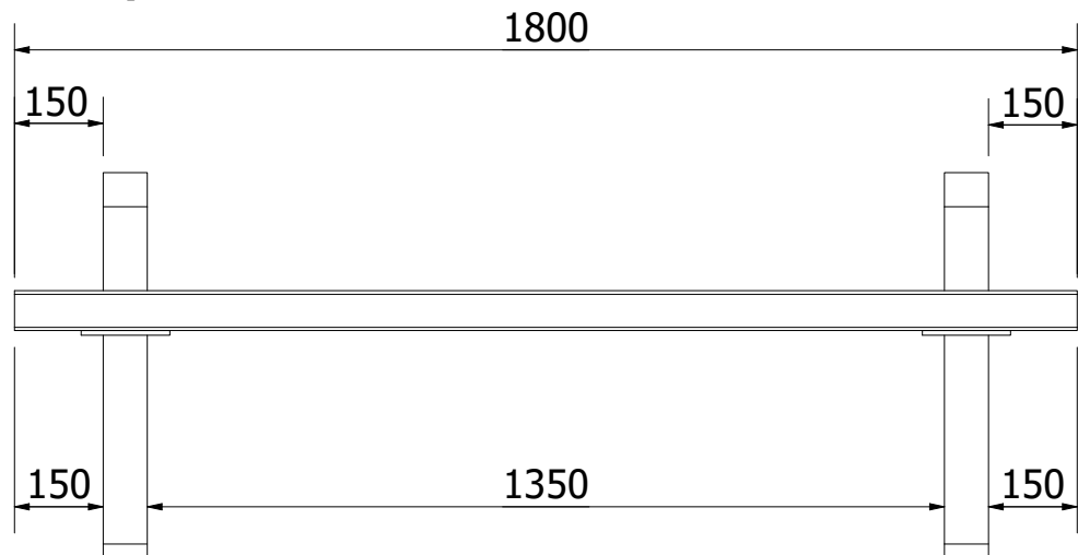
FRONT VIEW ( 1 : 14 )
