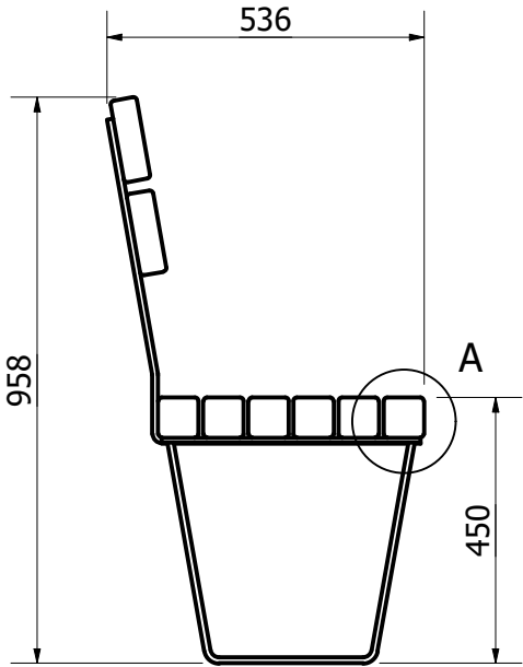
SIDE VIEW ( 1 : 14 )
