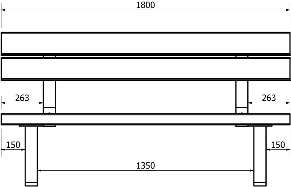
FRONT VIEW ( 1 : 14 )
