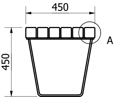
SIDE VIEW ( 1 : 14 )
