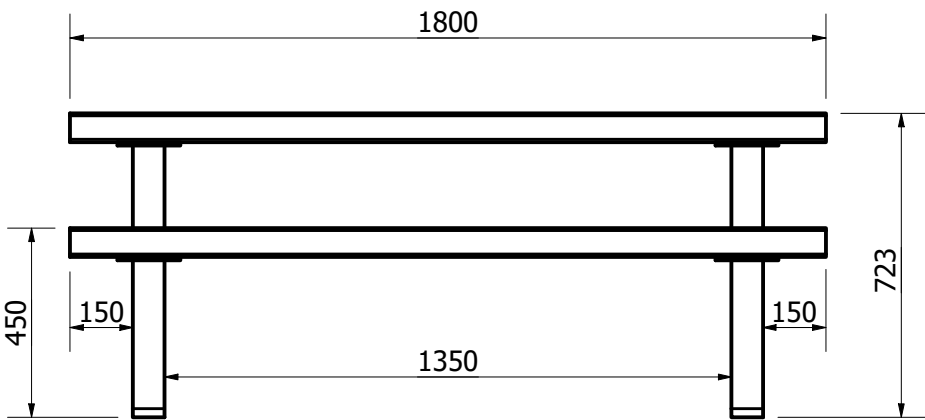
FRONT VIEW ( 1 : 18 )
