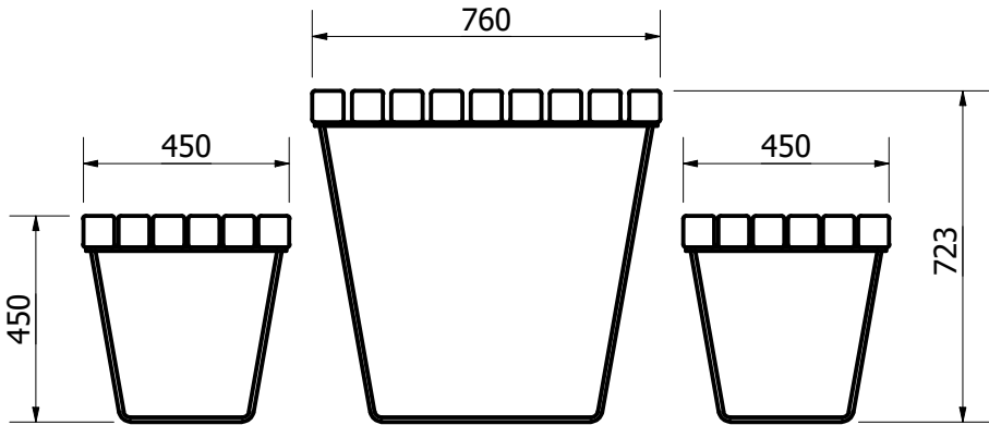
SIDE VIEW ( 1 : 18 )
