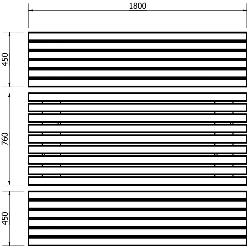
TOP VIEW ( 1 : 18 )
