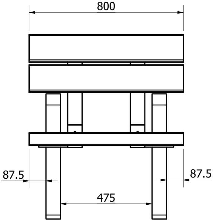
FRONT VIEW ( 1 : 12 )
