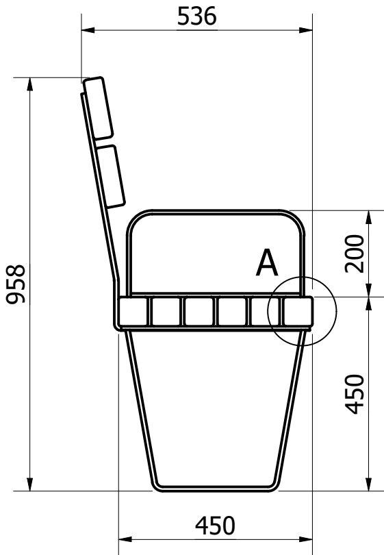
SIDE VIEW ( 1 : 12 )
