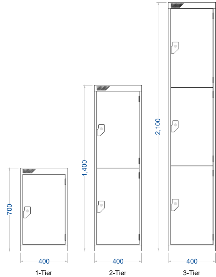
Front View
