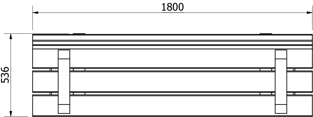
TOP VIEW ( 1 : 14 )
