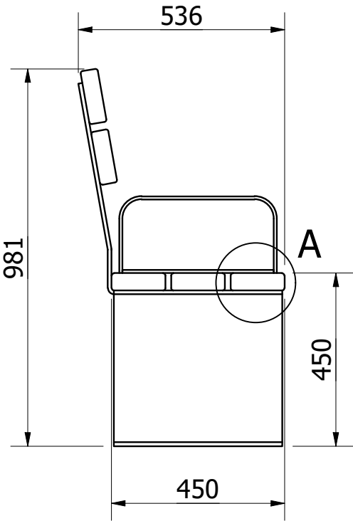
SIDE VIEW ( 1 : 14 )
