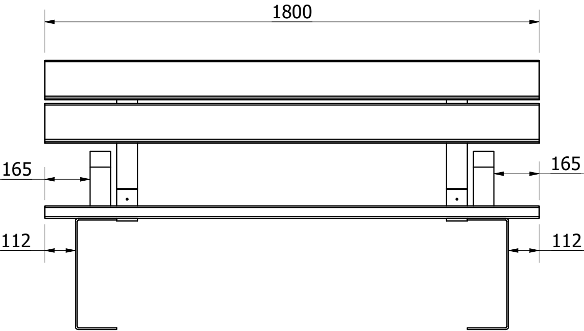
FRONT VIEW ( 1 : 14 )
