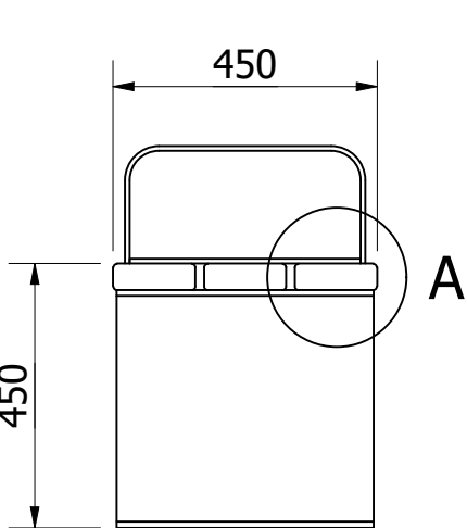
SIDE VIEW ( 1 : 14 )
