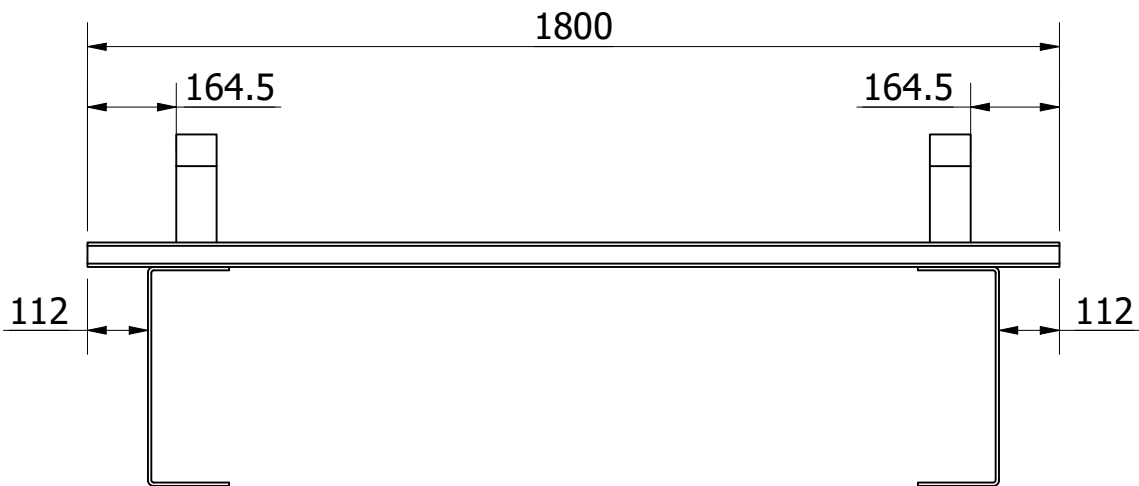
FRONT VIEW ( 1 : 14 )
