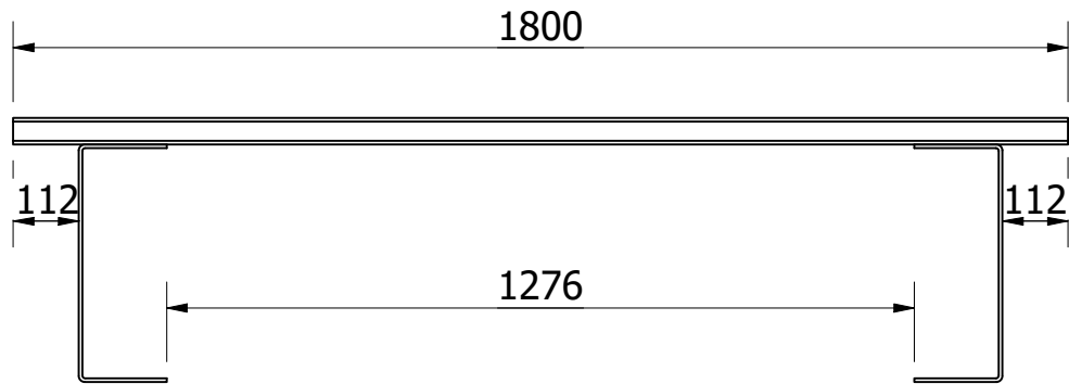
FRONT VIEW ( 1 : 14 )
