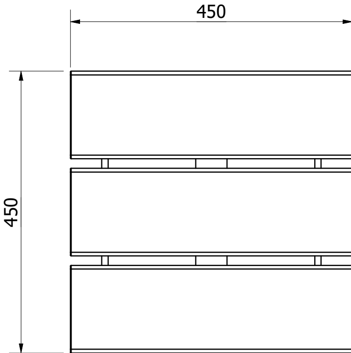
TOP VIEW ( 1 : 6 )
