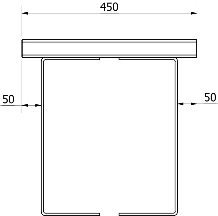
FRONT VIEW ( 1 : 6 )
