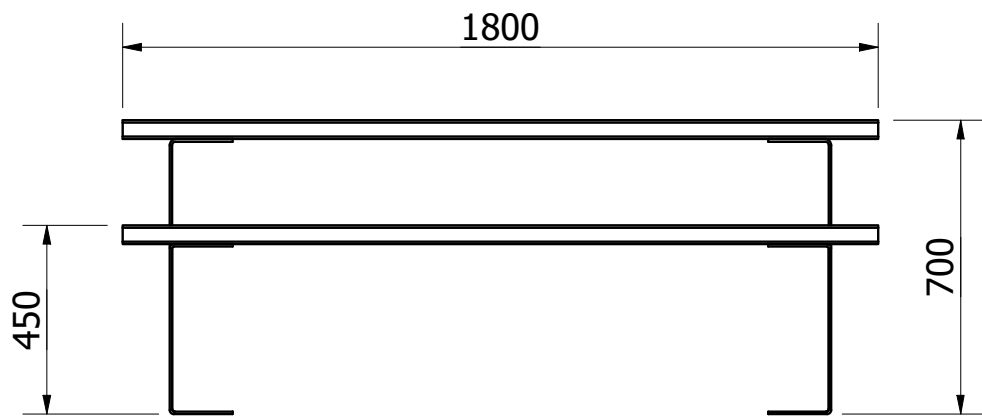
FRONT VIEW ( 1 : 18 )
