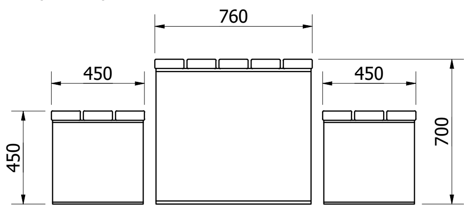
SIDE VIEW ( 1 : 18 )
