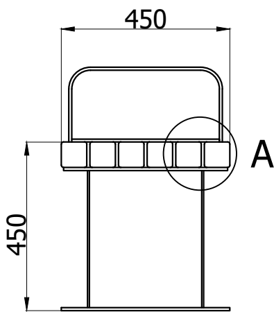
SIDE VIEW ( 1 : 14 )
