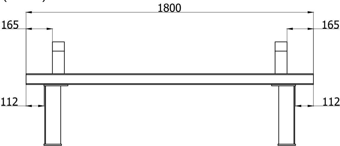
FRONT VIEW ( 1 : 14 )
