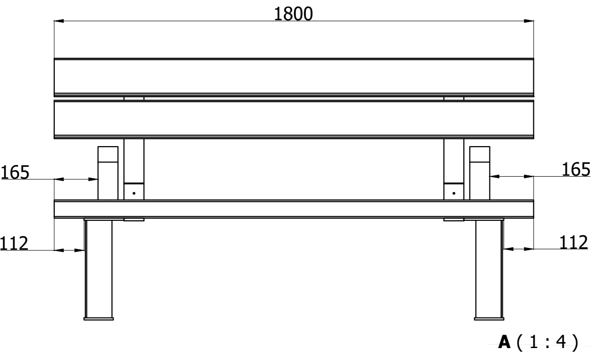
FRONT VIEW ( 1 : 14 )
