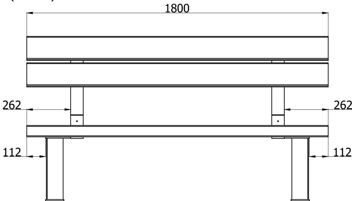
FRONT VIEW ( 1 : 14 )
