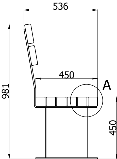
SIDE VIEW ( 1 : 14 )
