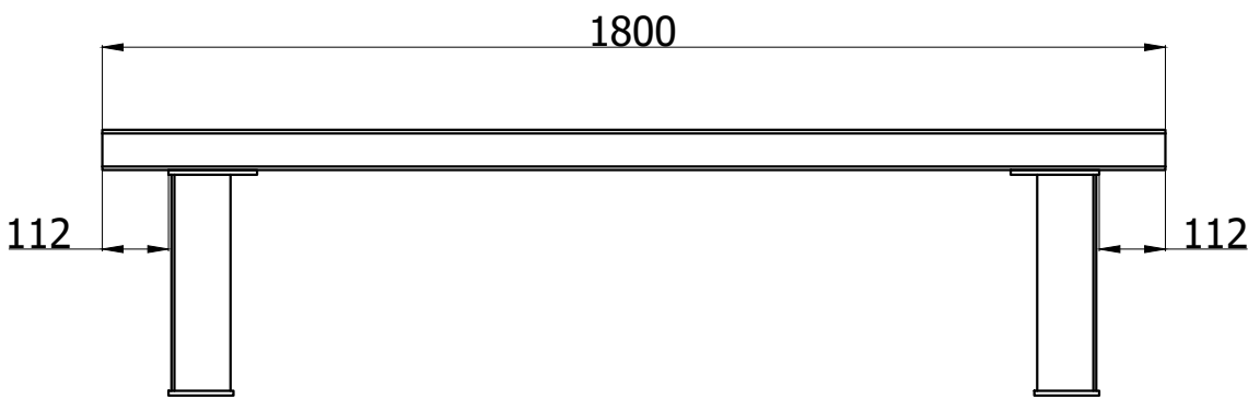
FRONT VIEW ( 1 : 14 )
