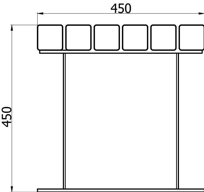
SIDE VIEW ( 1 : 6 )
