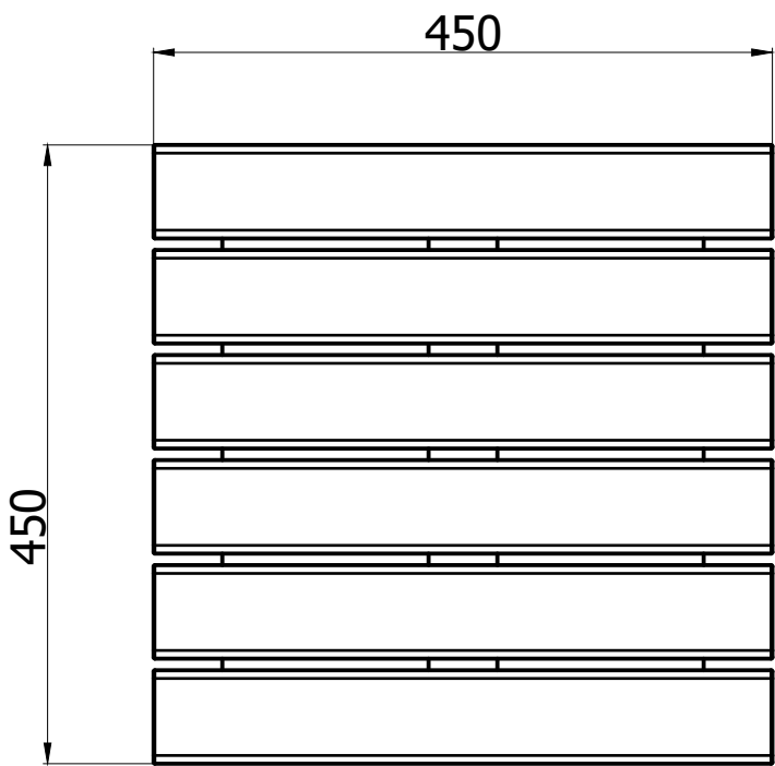
TOP VIEW ( 1 : 6 )
