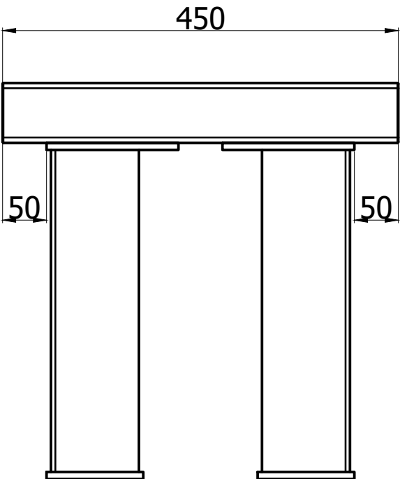
FRONT VIEW ( 1 : 6 )
