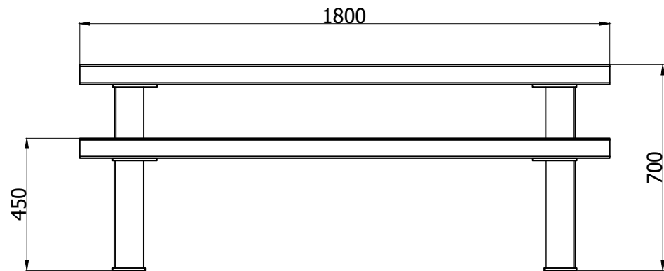
FRONT VIEW ( 1 : 18 )
