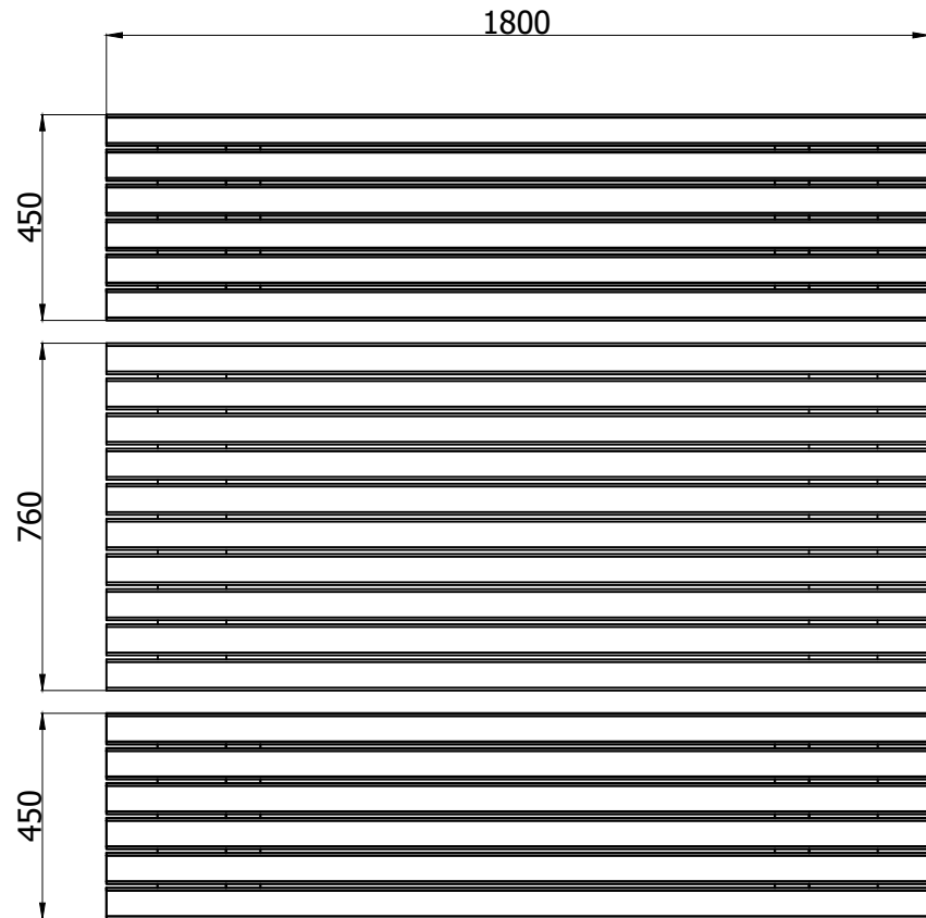
TOP VIEW ( 1 : 18 )
