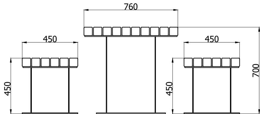
SIDE VIEW ( 1 : 18 )
