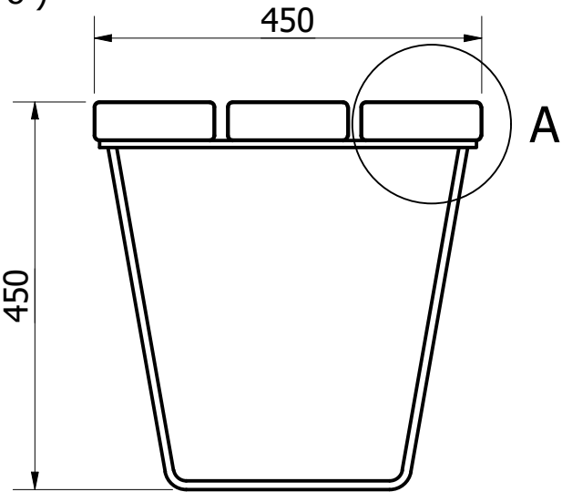
SIDE VIEW ( 1 : 8 )
