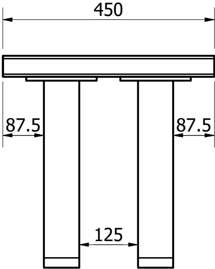
FRONT VIEW ( 1 : 8 )
