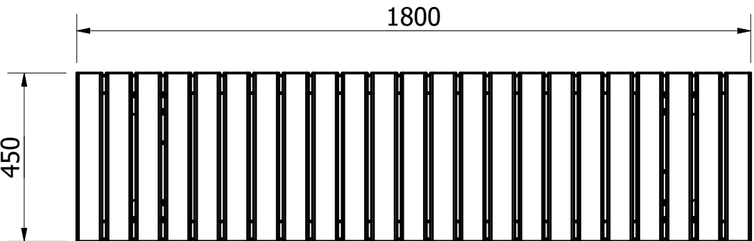
TOP VIEW ( 1 : 14 )
