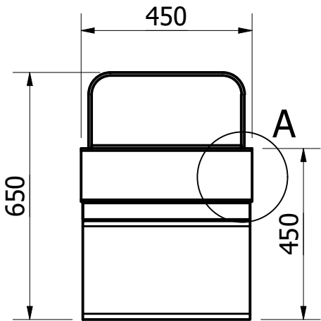
SIDE VIEW ( 1 : 14 )
