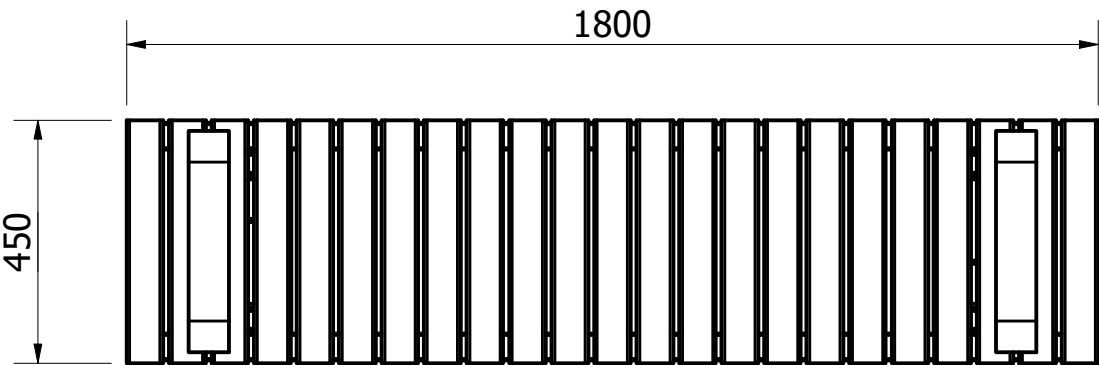
TOP VIEW ( 1 : 14 )
