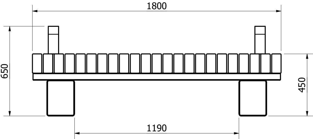
FRONT VIEW ( 1 : 14 )
