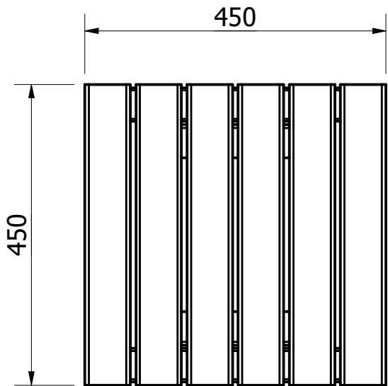
TOP VIEW ( 1 : 8 )
