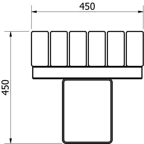
FRONT VIEW ( 1 : 8 )
