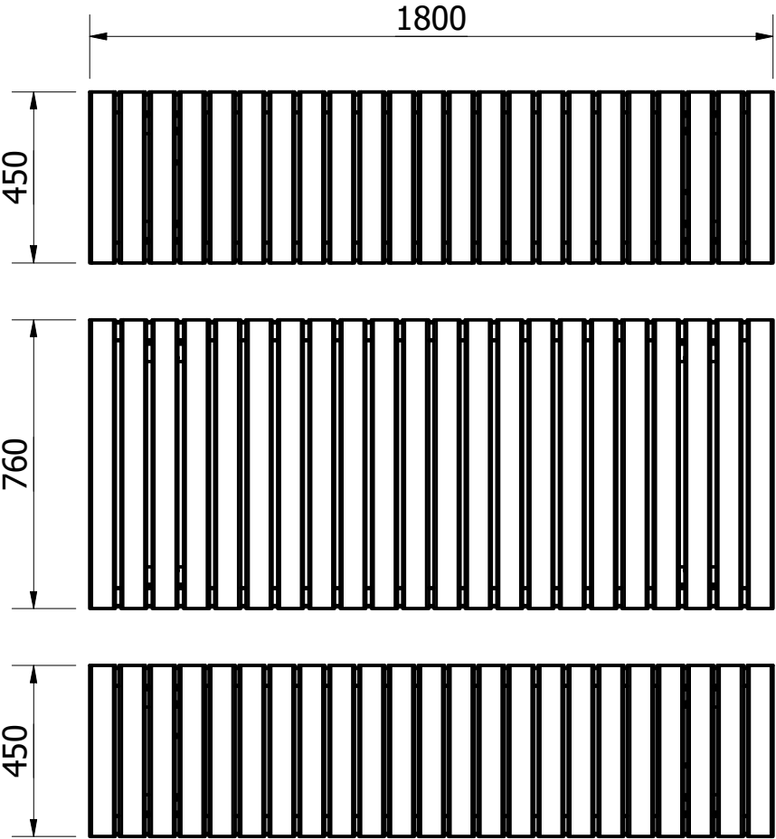
TOP VIEW ( 1 : 18 )
