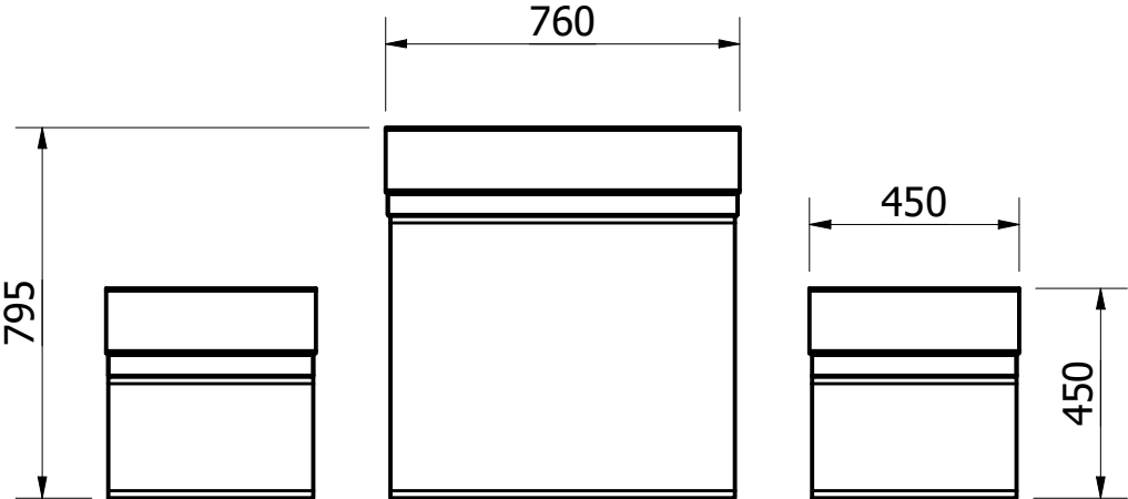
SIDE VIEW ( 1 : 18 )
