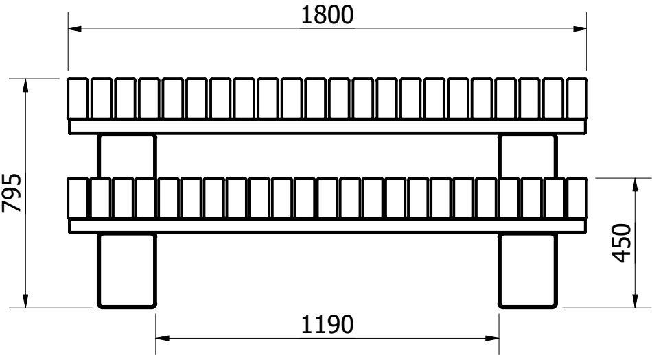
FRONT VIEW ( 1 : 18 )
