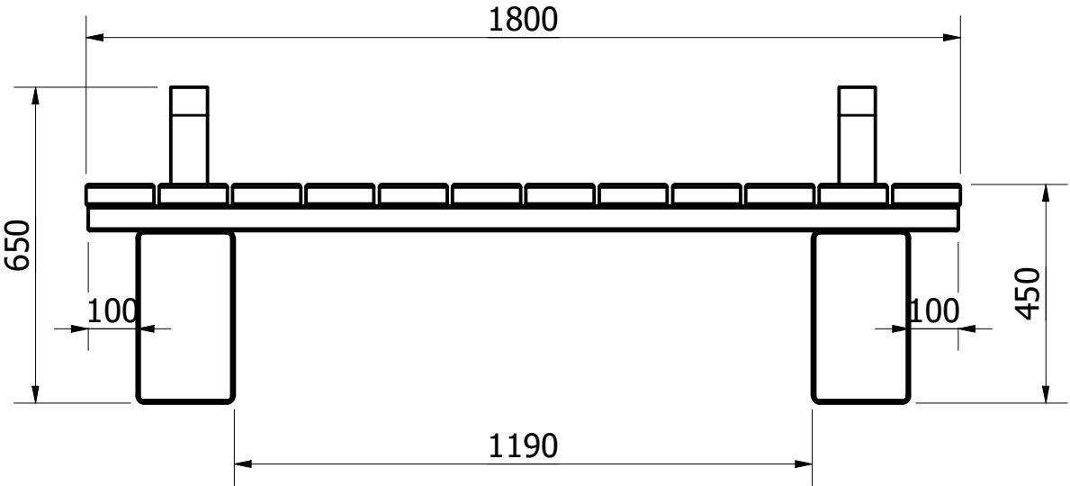
FRONT VIEW ( 1 : 14 )
