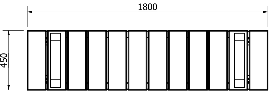
TOP VIEW ( 1 : 14 )
