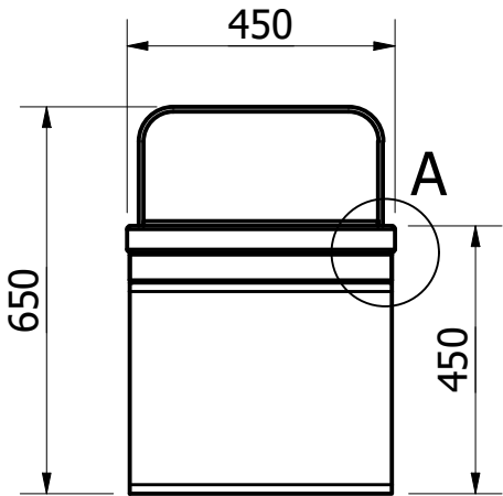
SIDE VIEW ( 1 : 14 )
