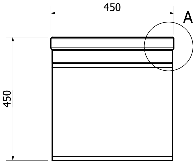
SIDE VIEW ( 1 : 8 )
