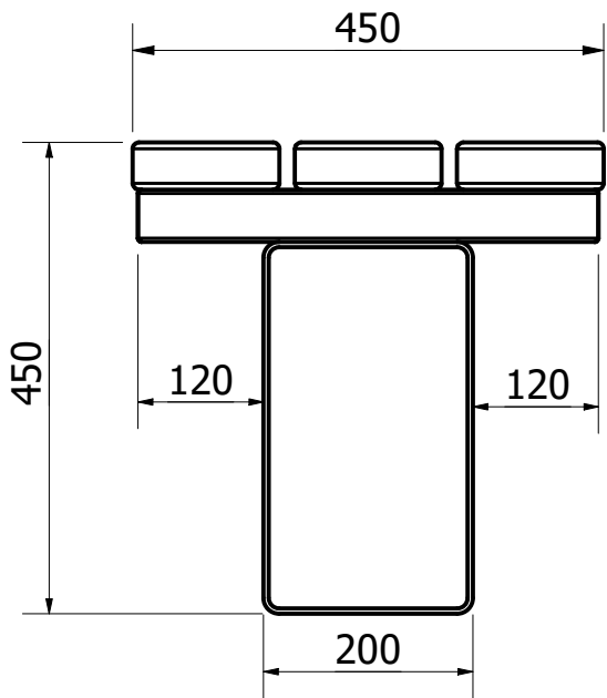
FRONT VIEW ( 1 : 8 )
